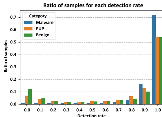
Figure 10: Amount of samples for the ratio of machines with anomalous file write (Using 1 random benign execution).
