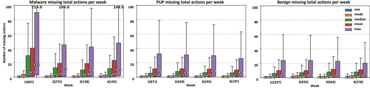
Figure 3: Missing actions compared to the previous week.
