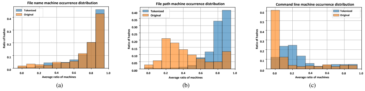
Figure 9: The average ratio of machines the parameter values appear on. The graphs show the average amount of machines the values of file name, file path and command line appear on. The orange color graphs are the full values of the parameters while the blue graphs are the token values.
