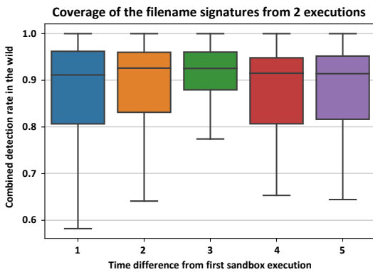
Figure 8: Total filename signature coverage for re-execution intervals. A periodic execution of every 3 weeks yields the highest coverage across all malware.
