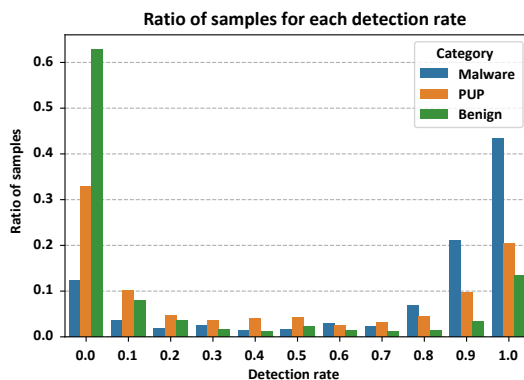
Figure 11: Amount of samples for the ratio of machines with anomalous file write (Using all benign execution).
